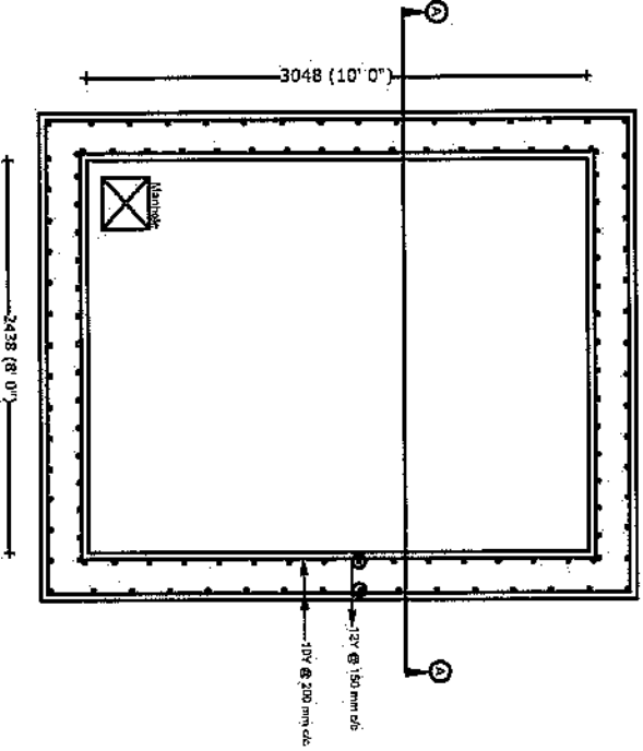
PLAN PLAN OF SLUMP (2.438m x 3.048m x 2.438m) (8'0" x 10'0" x 8'0") 16,000 Litres Capacity
