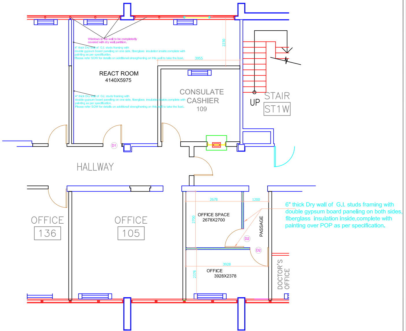
PROPOSED PARTITION WALL LAYOUT
