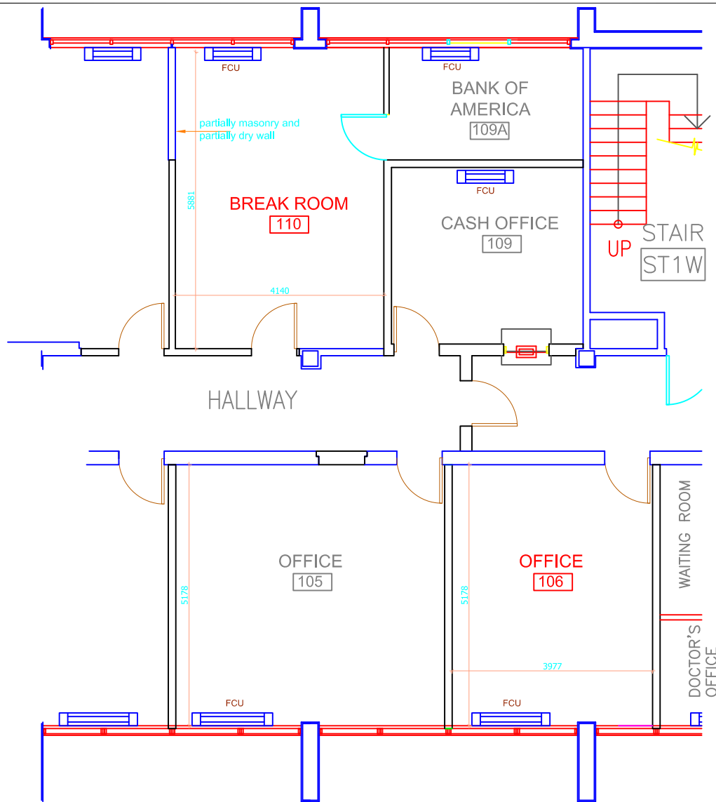
PART FLOOR PLAN OF 1ST FLOOR SHOWING EXISTING LAYOUT
